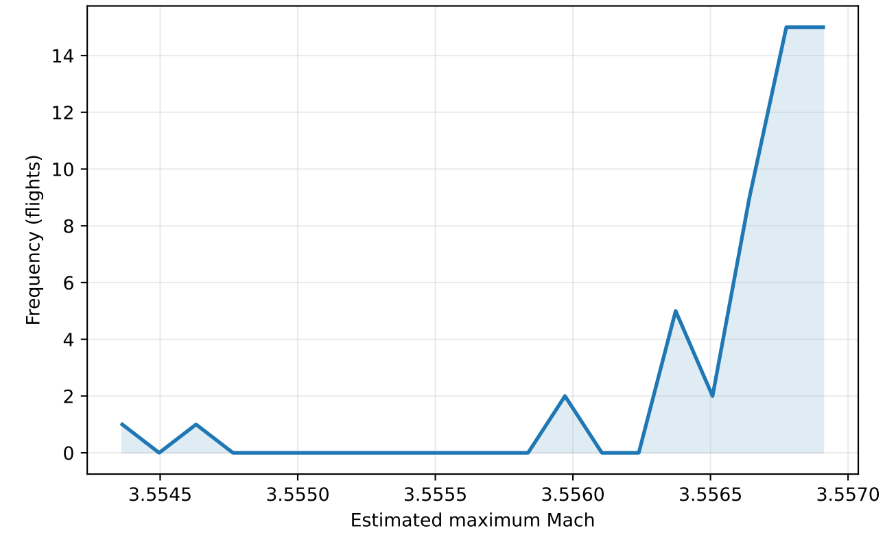
Maximum Mach Frequency
